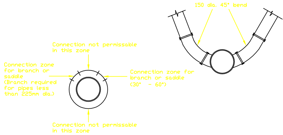
SECTION THROUGH EXISTING DRAIN
