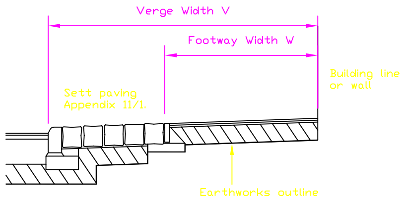
FOOTWAY TYPE F2 (A,B,C,D & E) (See note 2)
