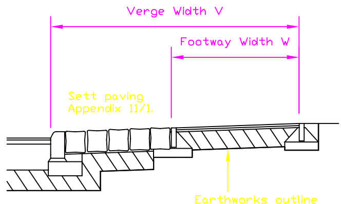
FOOTWAY TYPE F4 (A,B,C,D & E) (See note 2)
