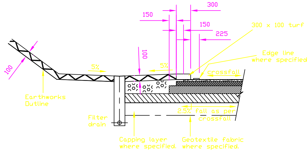
CUTTING
