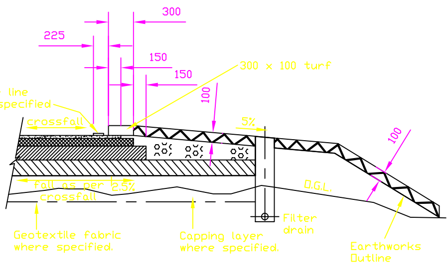
LOW EMBANKMENT
