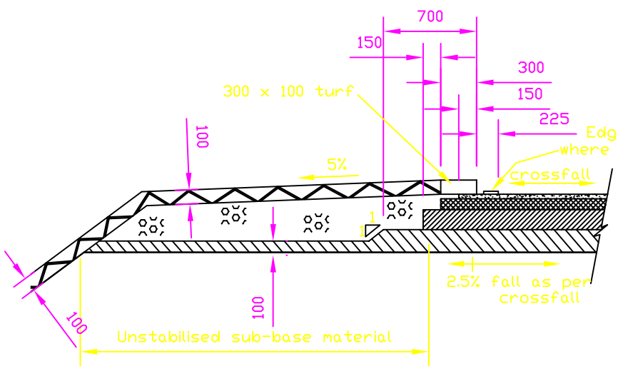
EMBANKMENT
